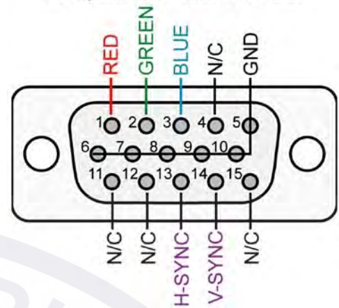
VGA port, view from Wire Side
