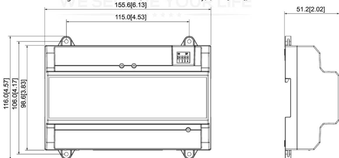
Figure 1-1 Dimensions (two-door one-way) (mm [inch])
