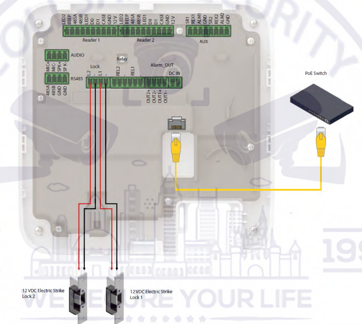
Figure 3-15 Wiring of locks
