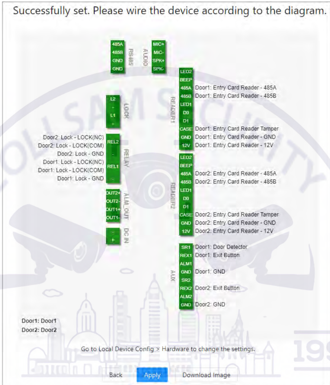
Figure 5-7 Wiring diagram
