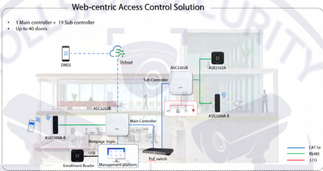
Figure 5-0 Networking diagram
