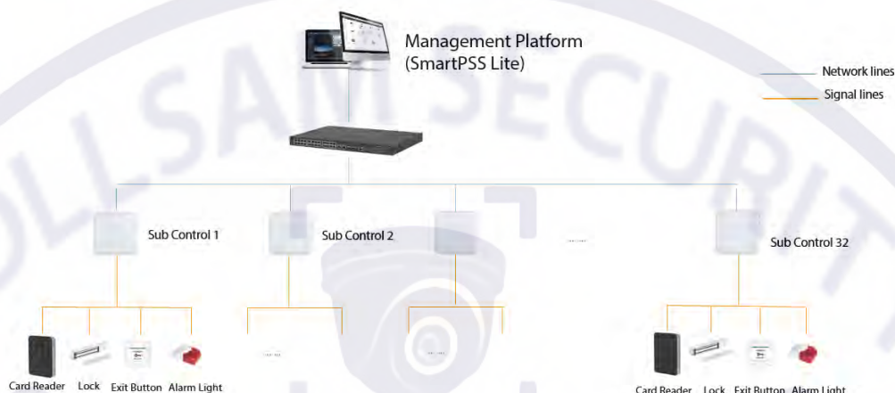
Figure 3-1 Networking Diagram
