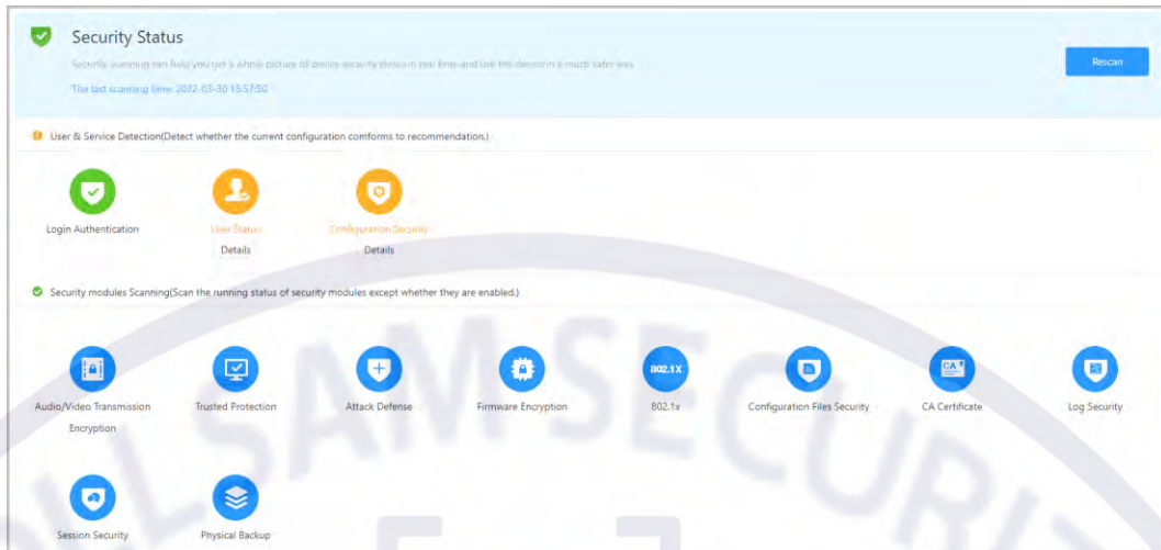
Figure 2-50 Security Status
