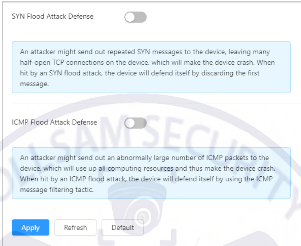
Figure 2-55 Anti-DoS attack
