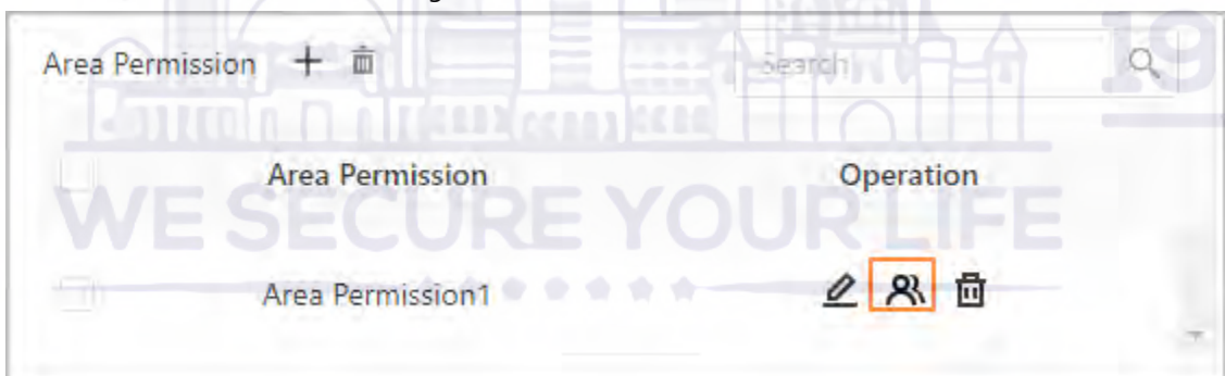
Figure 2-20 Select users
