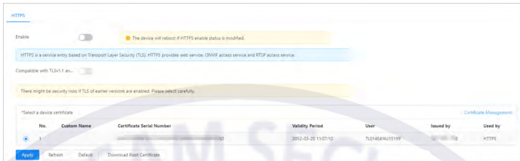
Figure 2-51 HTTPS
