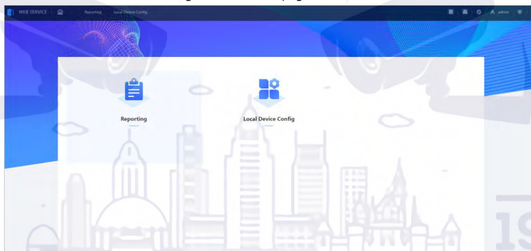
Figure 2-61 Home page
