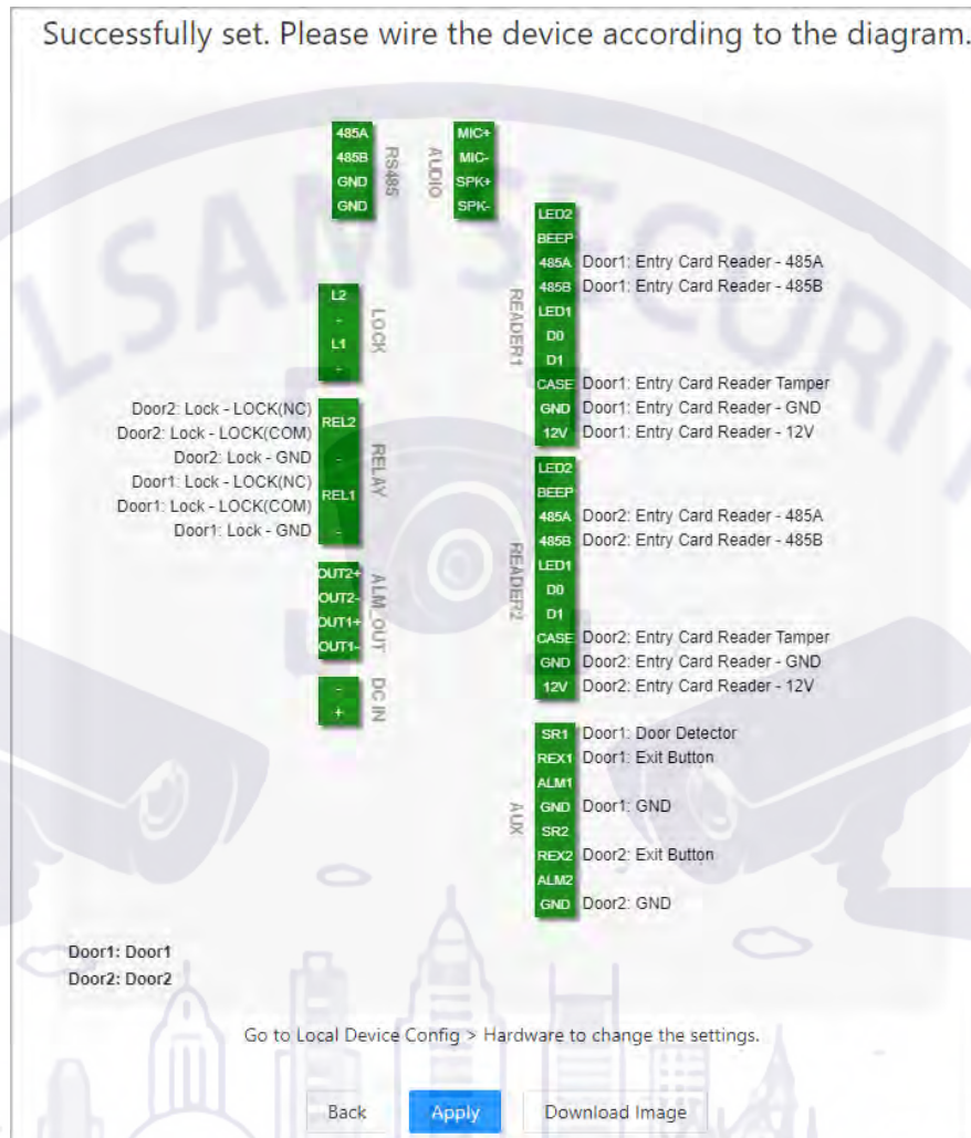
Figure 2-8 Wiring diagram
