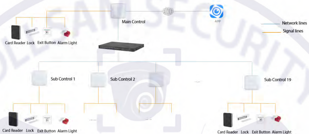
Figure 2-1 Networking diagram
