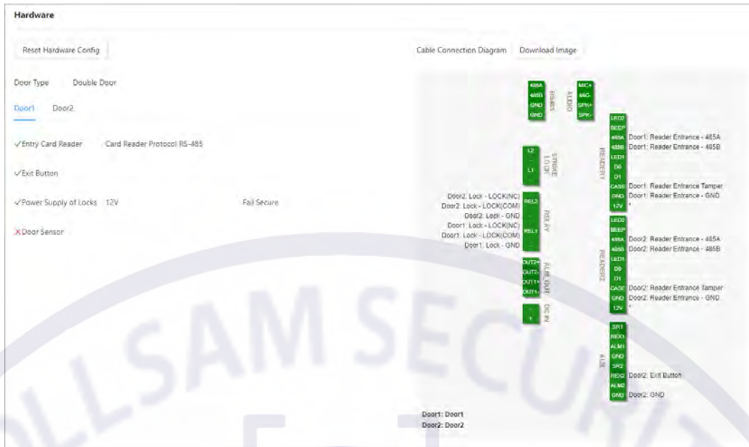
Figure 2-47 Hardware
