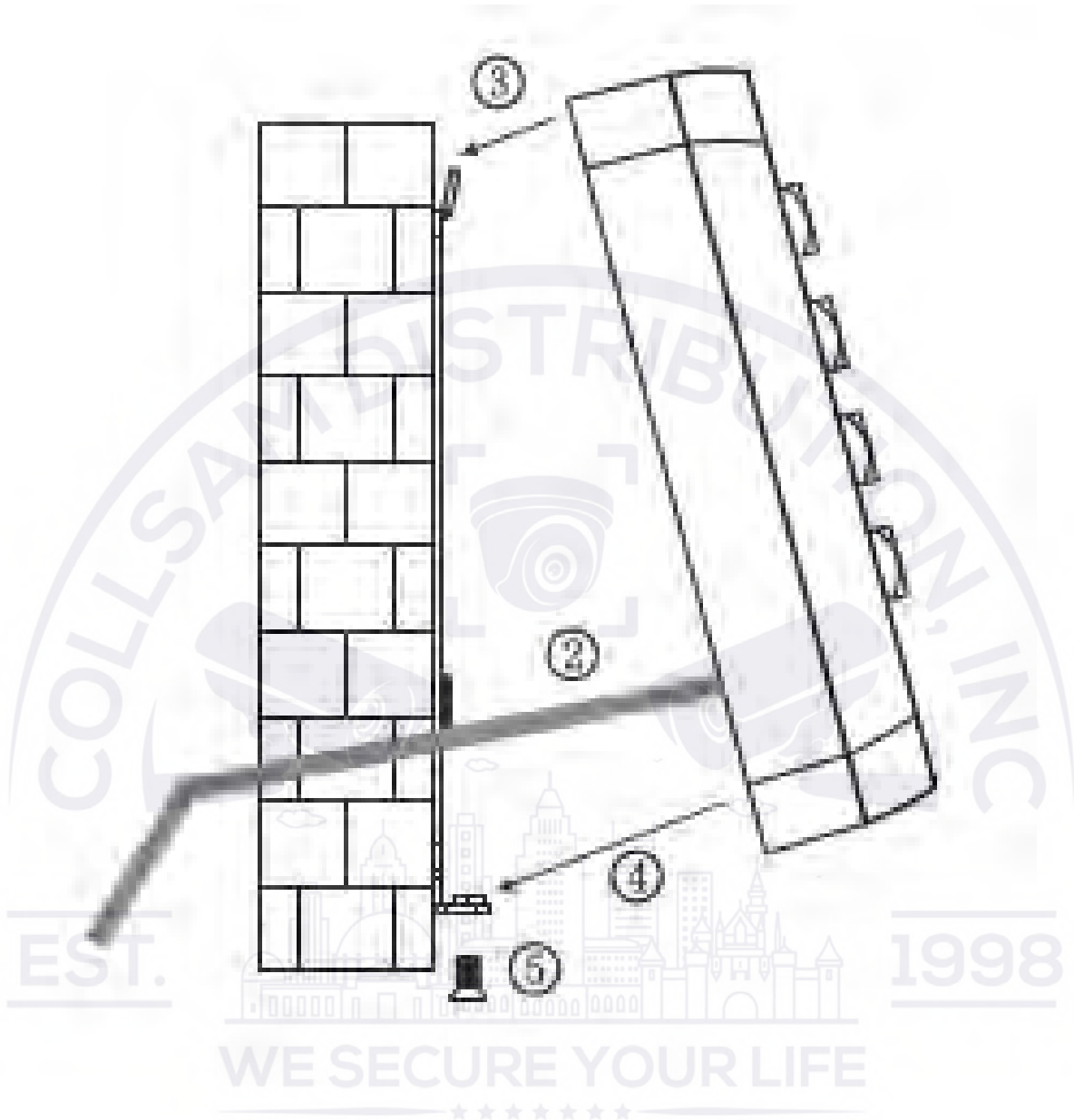
Figure 3-1 Installation
