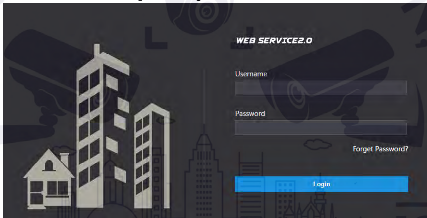
Figure 4-2 Login interface
