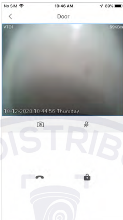
Figure 5-4 Door
