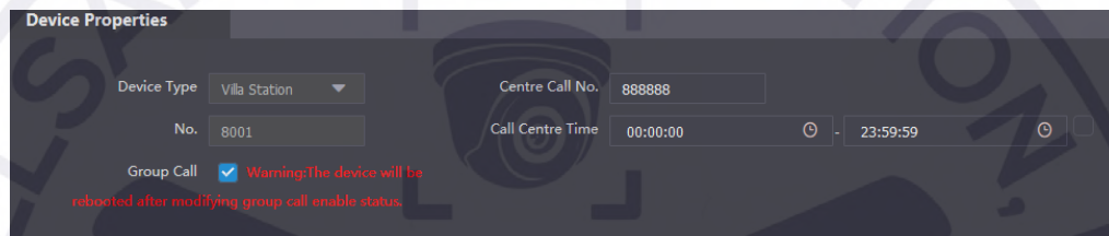
Figure 4-4 Device properties
