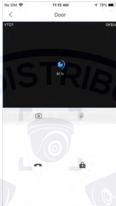
Figure 5-13 Door
