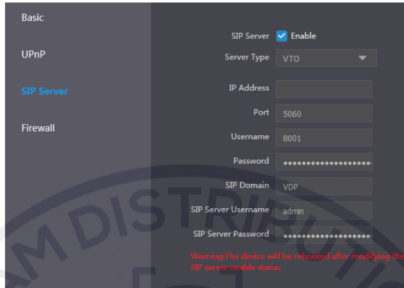
Figure 4-6 SIP server
