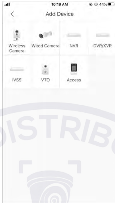
Figure 5-2 Add device
