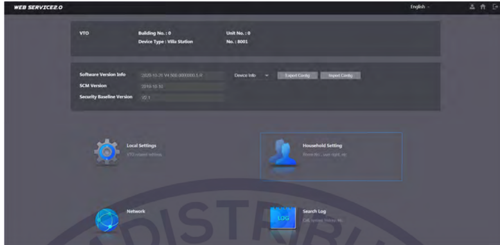
Figure 4-3 Main interface
