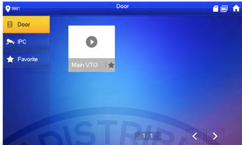
Figure 4-13 Door
