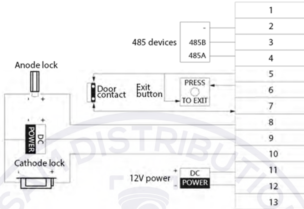
Figure 2-8 Cable connection
