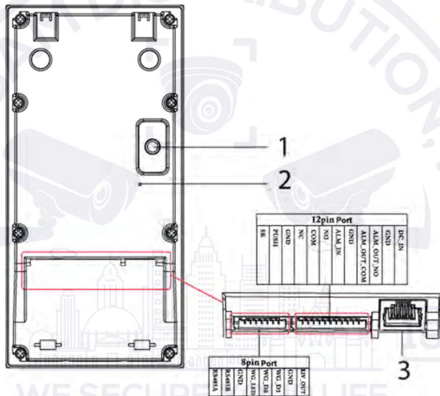
Figure 2-13 VTO3221E-P
