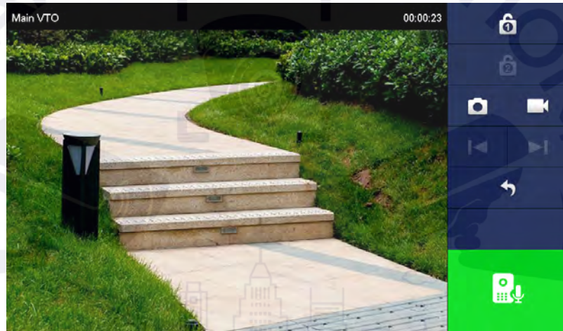
Figure 4-14 Monitoring video
