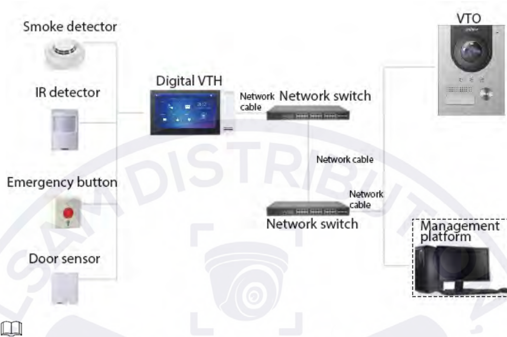
Figure 1-1 Network diagram
