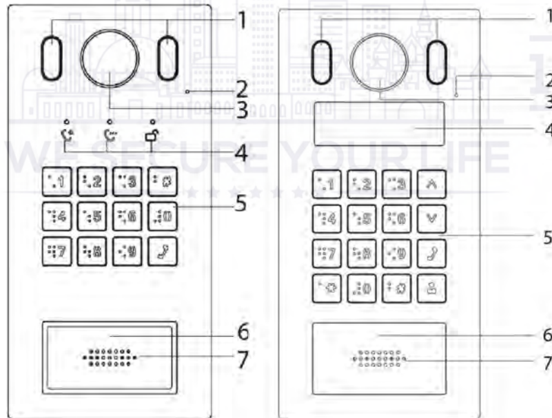
Figure 2-12 VTO3221E-P/ VTO6221E-P
