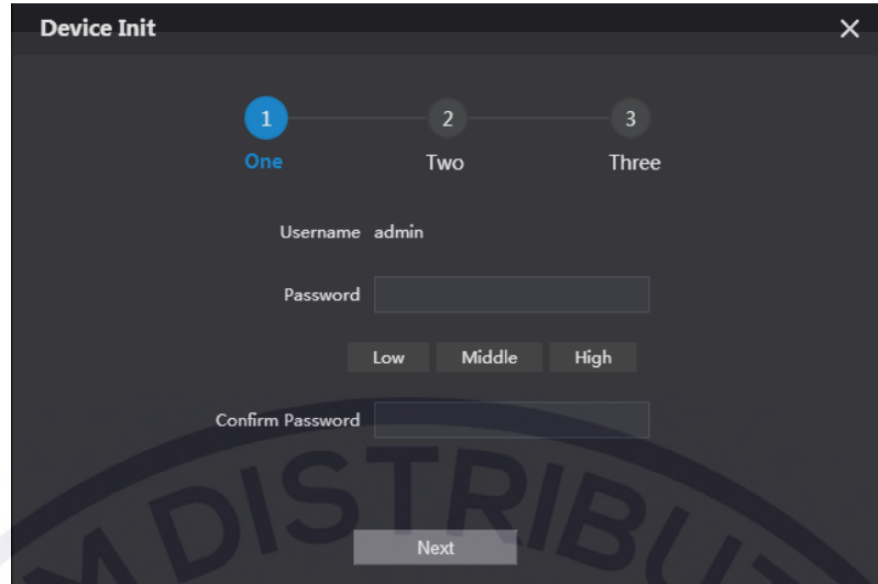
Figure 4-1 Device initialization
