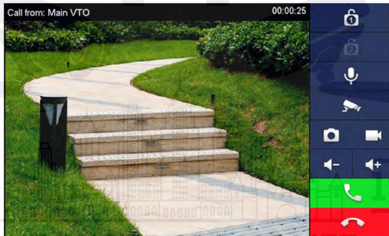
Figure 4-12 Call screen
