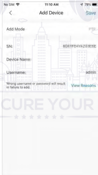
Figure 5-12 Add device
