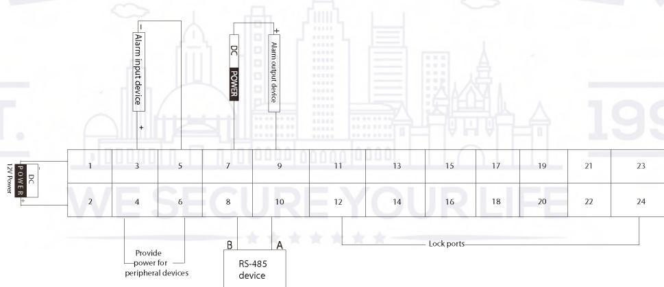
Figure 2-16 VTO2211G-P cable connection
