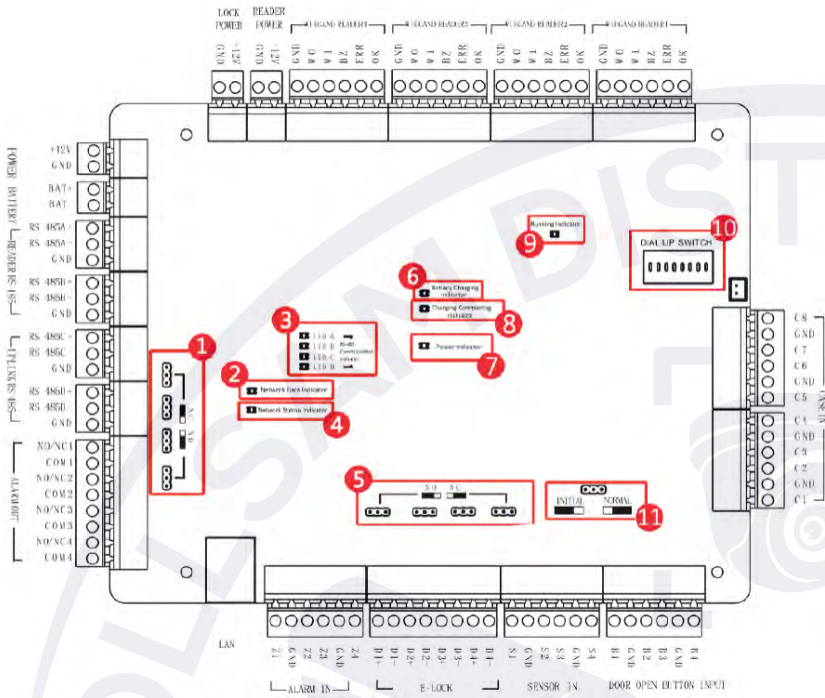
DS-K2604-G Network Access Controller
