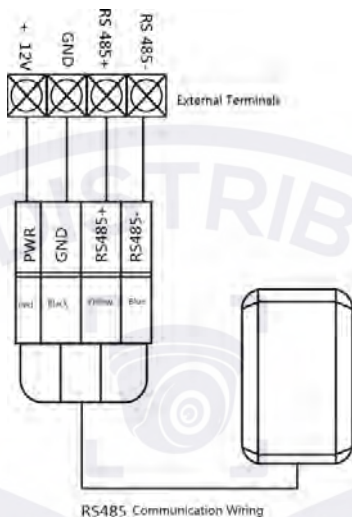
Figure 3-8 Wiring diagram of RS-485
