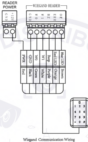
Figure 3-7 Wiring diagram of Wiegand card reader
