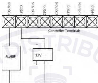
Figure 3-11 External Alarm Device Connection
