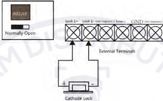
Figure 3-9 Wiring diagram of cathode lock
