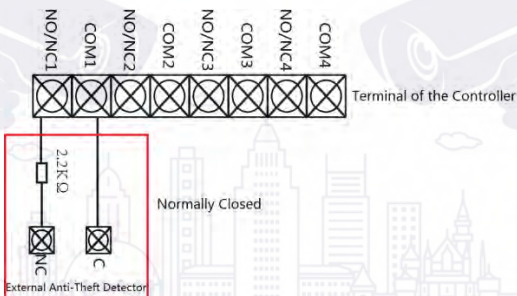
Figure 3-16 Normally Closed Status
