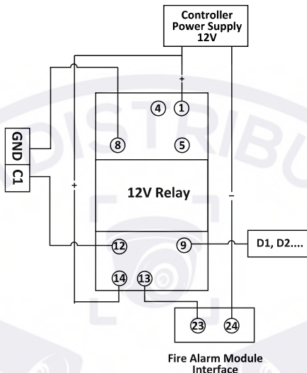
Figure 3-17 Fire Alarm Module Wiring
