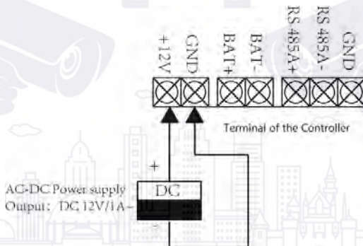
Figure 3-14 Power Supply Connection
