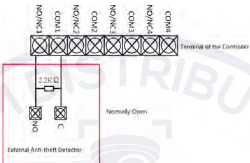
Figure 3-15 Normally Open Status
