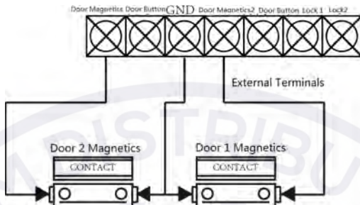
Figure 3-13 Magnetics Connection
