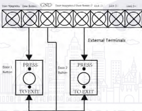
Figure 3-12 Power Button Connection
