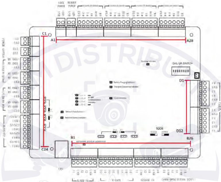
Figure 3-3 DS-K2604-G Access Controller Terminals
