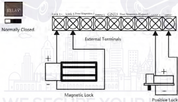
Figure 3-10 Wiring diagram of anode lock
