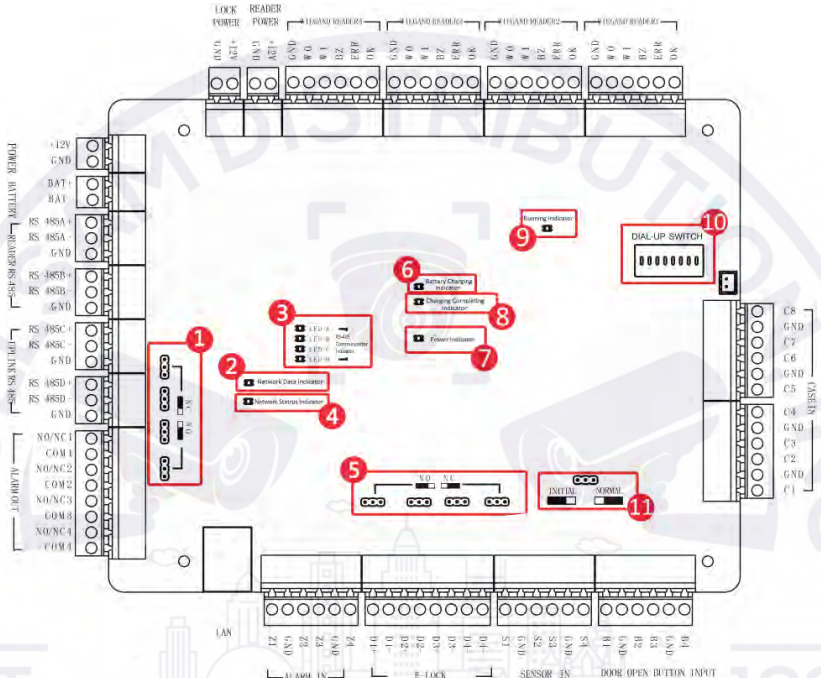
Figure 2-1 DS-K2604-G Component Schematic Diagram
