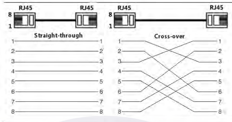
Figure 4-3 Connect cable
