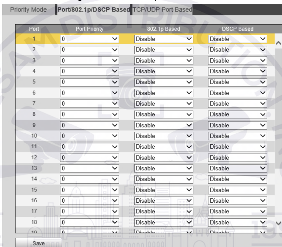
Figure 4-18 Port/802.1p/DSCP
