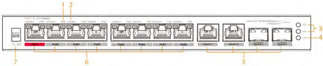
Figure 2-1 Front panel (with optical ports)
