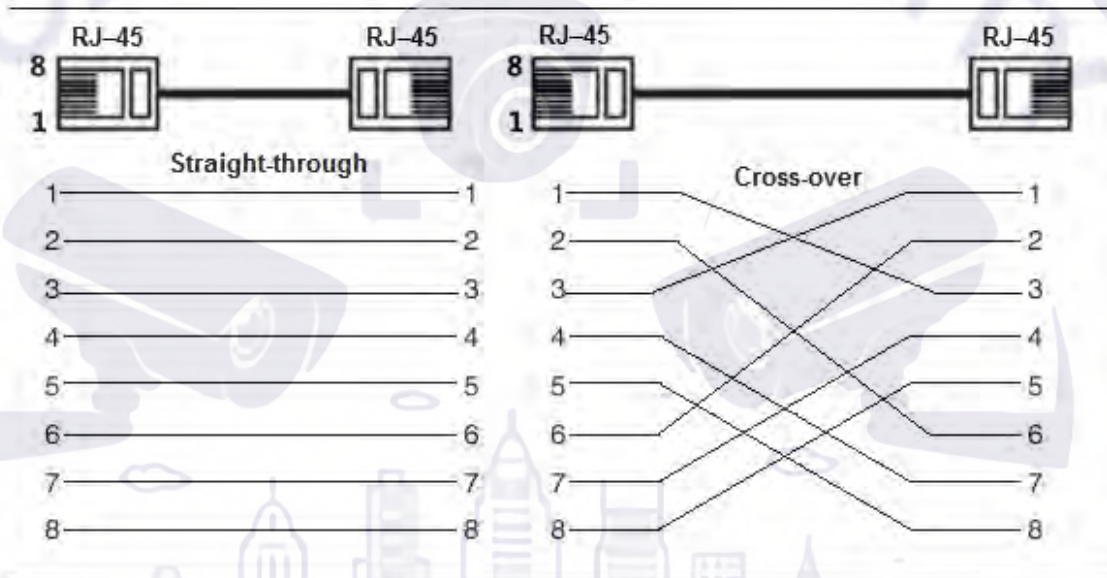
Figure 4-5 Pin description
