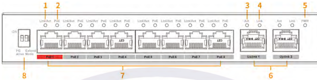
Figure 2-1 Front panel (without optical ports)
