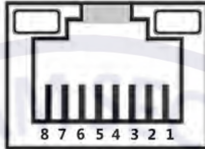
Figure 4-5 Pin description
