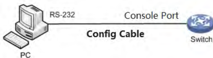
Figure 1-1 Networking
