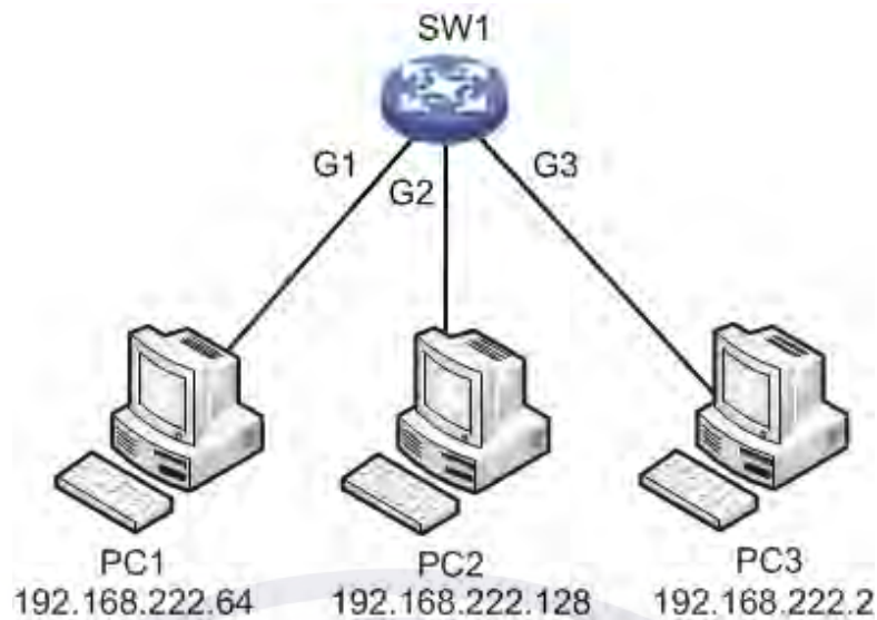
Figure 6-5 Networking
