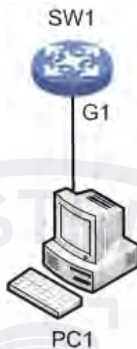
Figure 8-2 Networking
