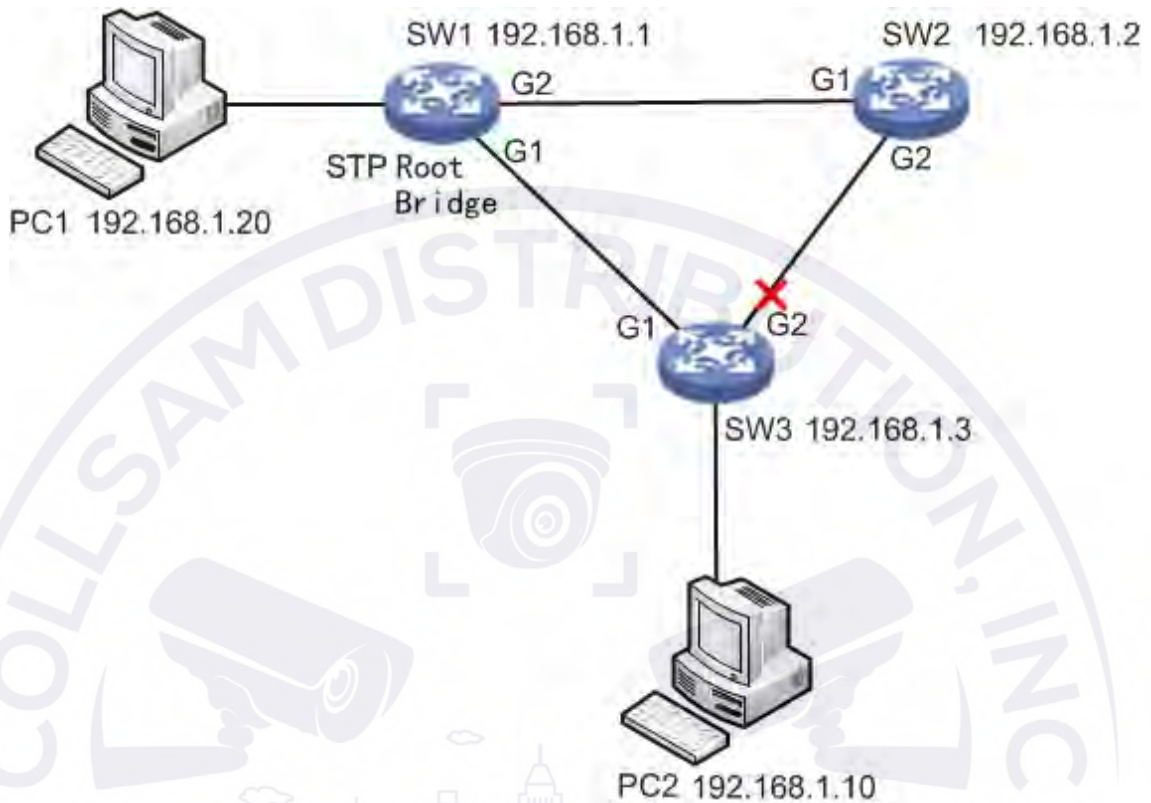
Figure 7-1 Networking
