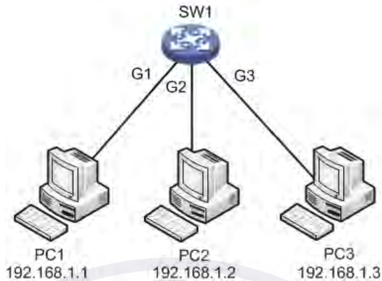
Figure 6-4 Networking
