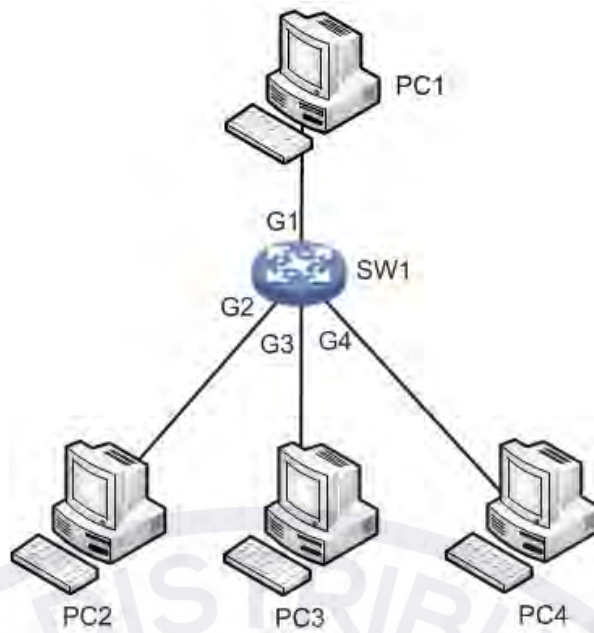
Figure 6-9 Networking
