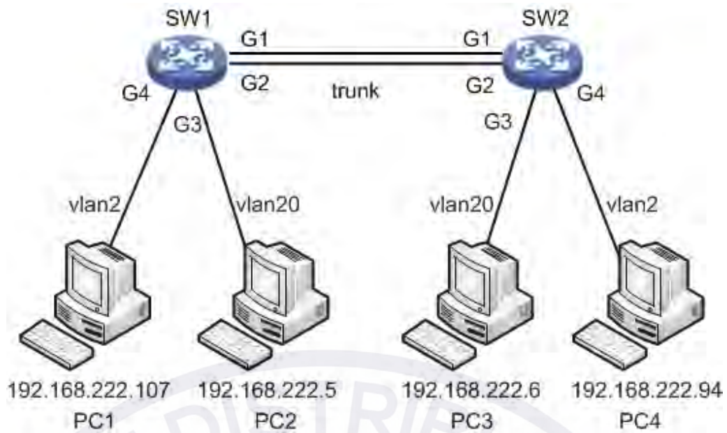
Figure 6-3 Networking
