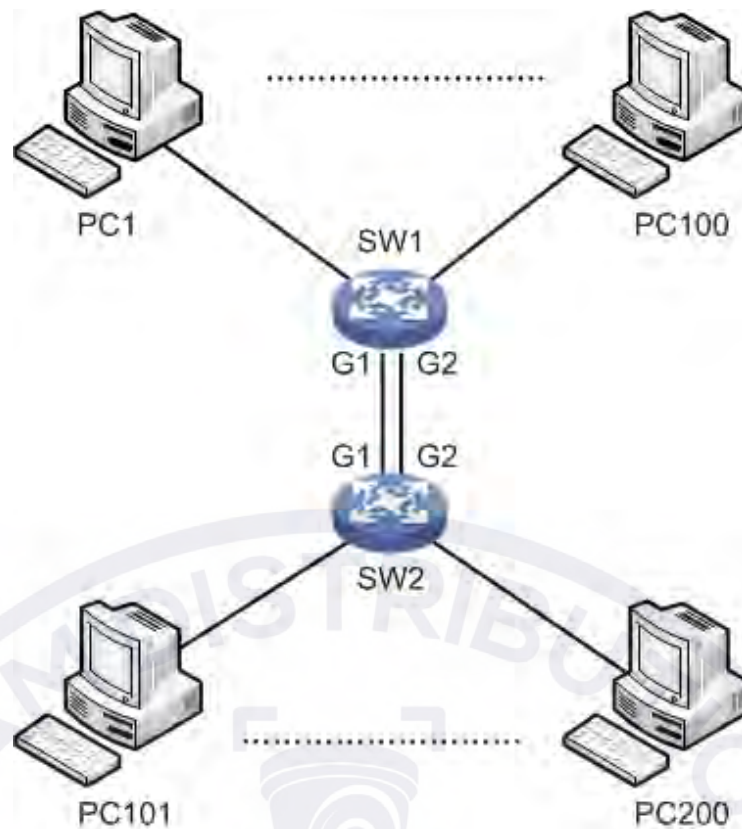
Figure 6-1 Networking
