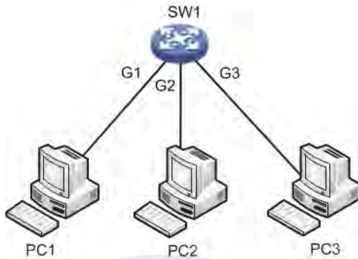
Figure 6-6 Networking
