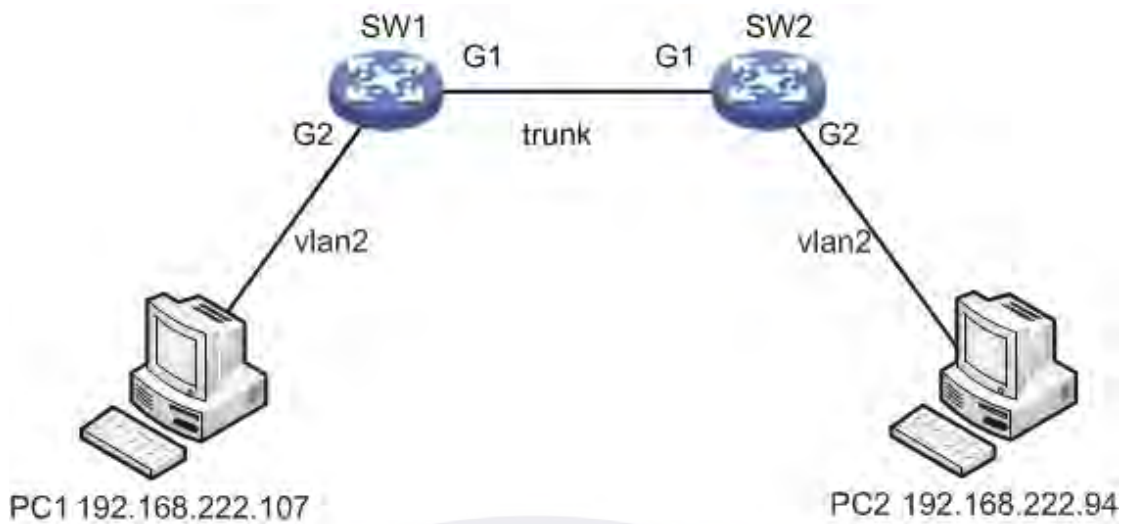
Figure 6-2 Networking
