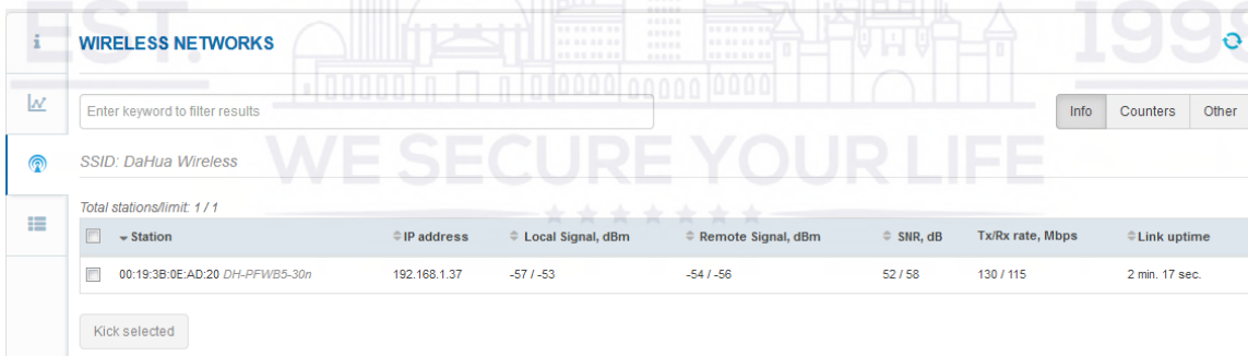
Figure 5 – Access Point's Wireless Statistics
