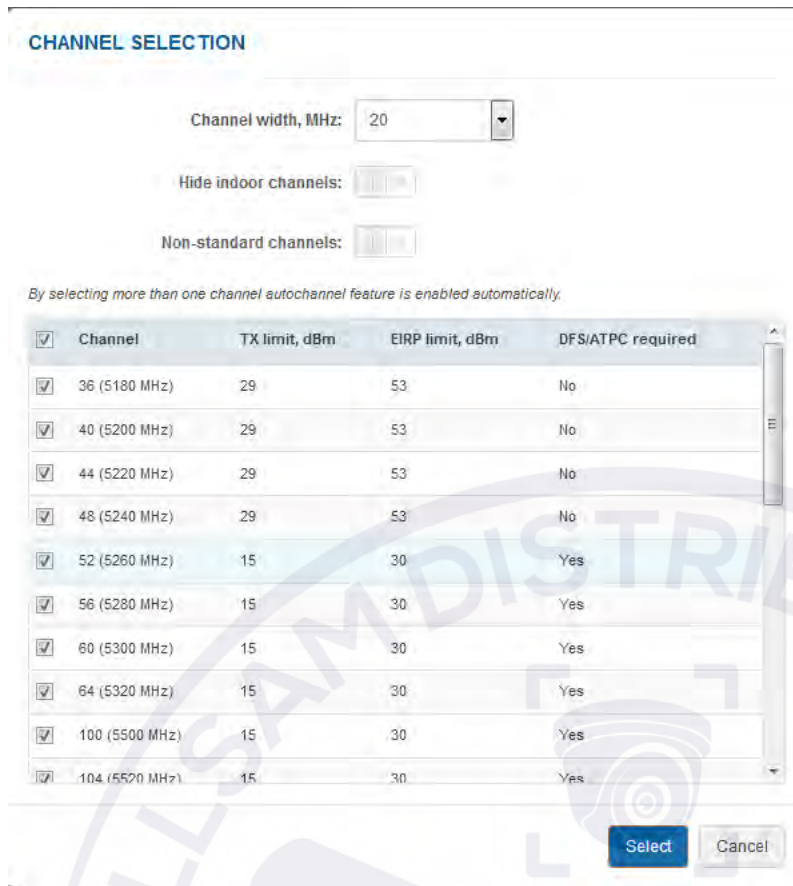
Figure 32 – Channel List Table
