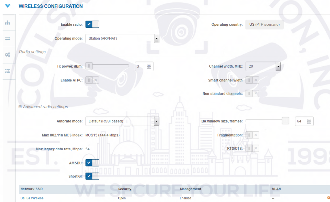
Figure 43 – Station Wireless Settings
