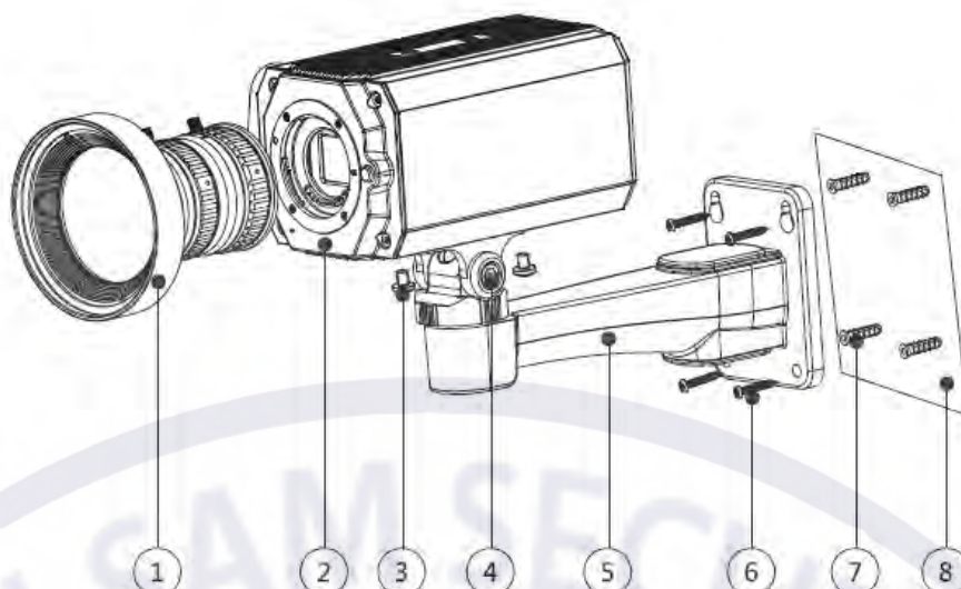
Figure 9-6 Device components
