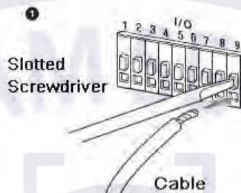
Figure 9-4 Install cable
