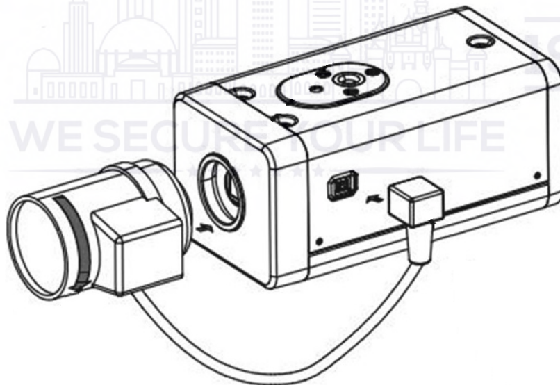
Figure 9-1 Lens installation (1)
