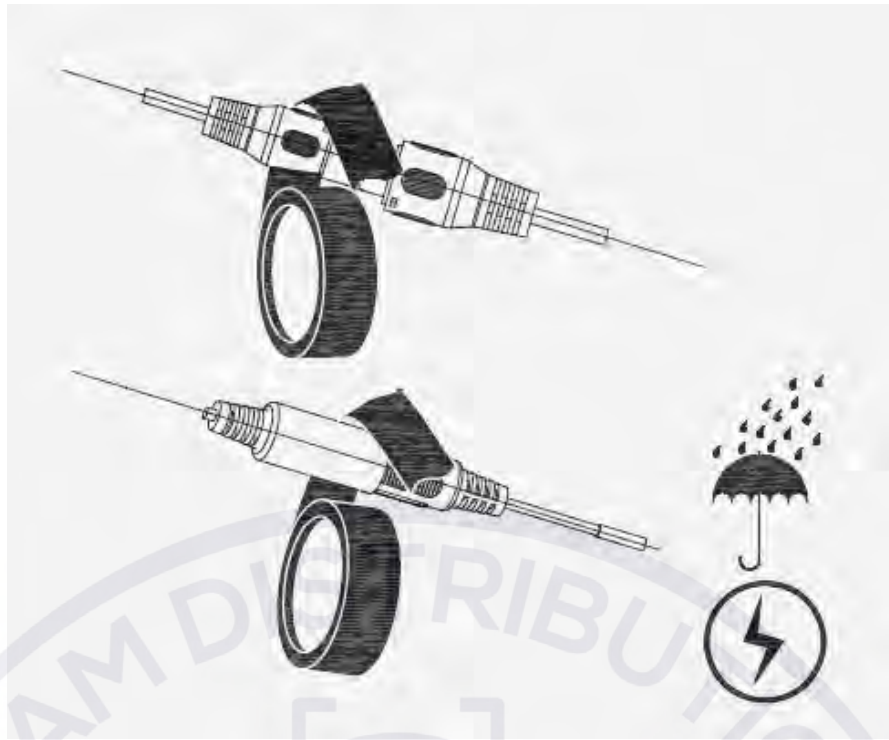
Figure 11-2 Waterproof measures
