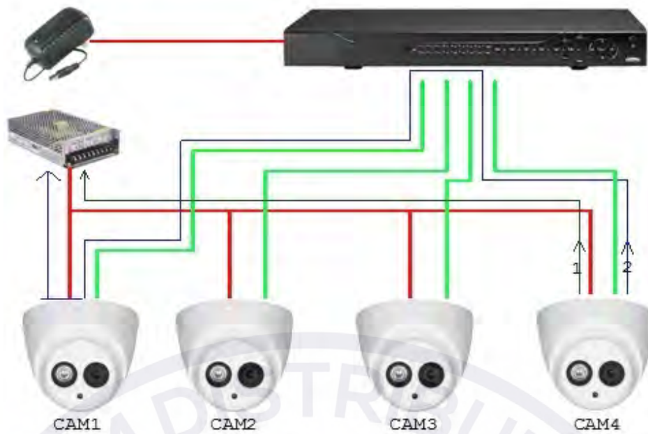
Figure 11-1 Principle of centralized power supply
