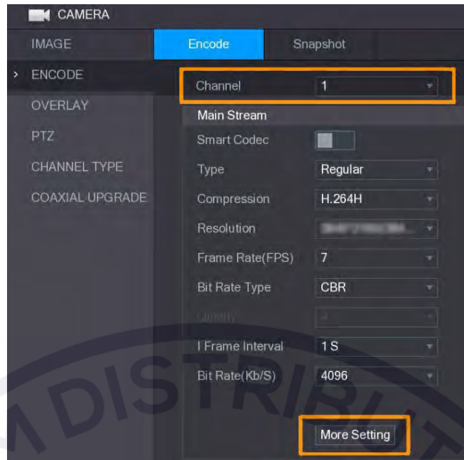
Figure 3-2 Encode setting
