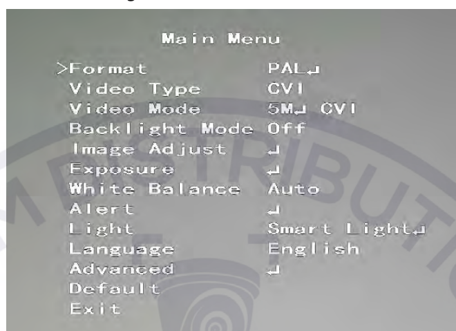
Figure 3-7 OSD menu
