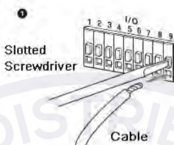
Figure 9-4 Install cable
