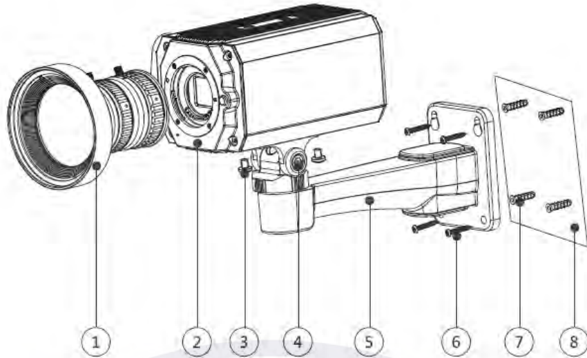
Figure 9-6 Device components
