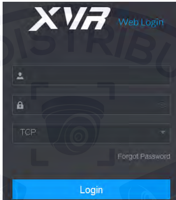
Figure 4-1 Login
