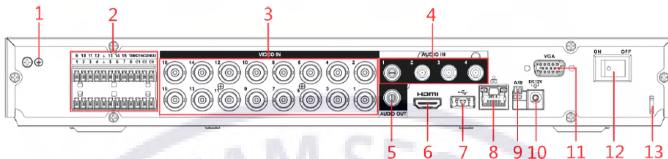
Figure 2-1 Rear panel
