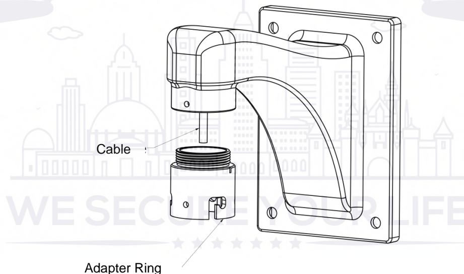
Figure 2 - 2: Locking the Pendant Adapter
