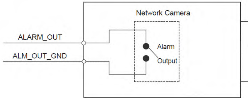
Figure 1-3 Alarm output
