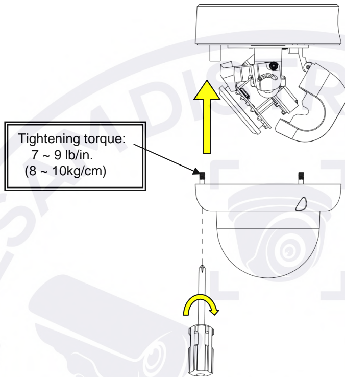
Figure 2 - 9: Assembling and Completing Camera Mounting
