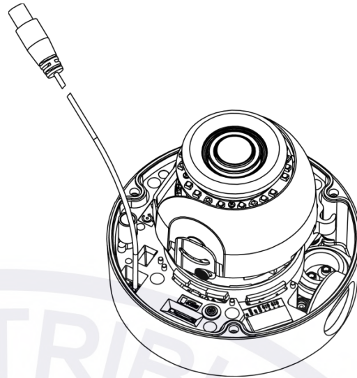
Figure 2 - 4: Connecting BNC Cable
