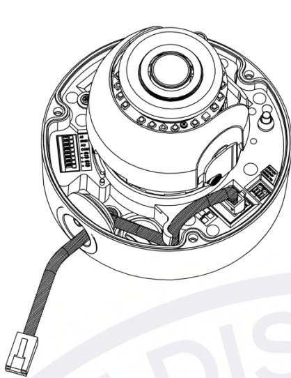
Figure 2 - 3: Connecting Ethernet Cable
