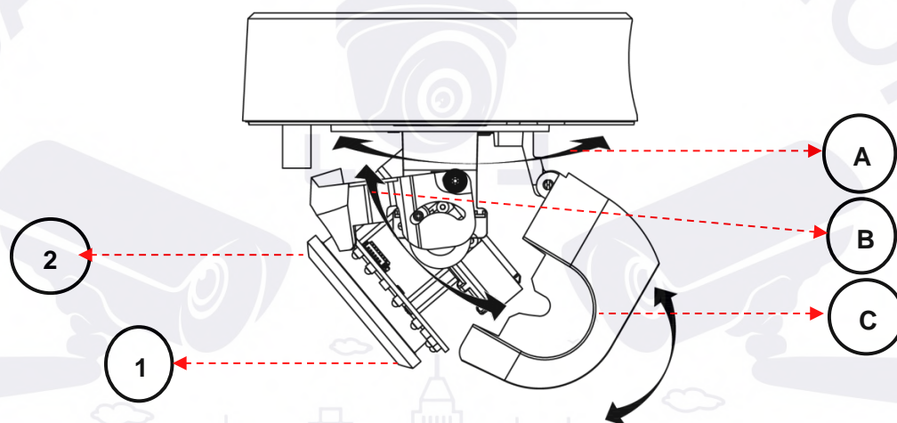
Figure 2 - 8: Positioning the Camera
