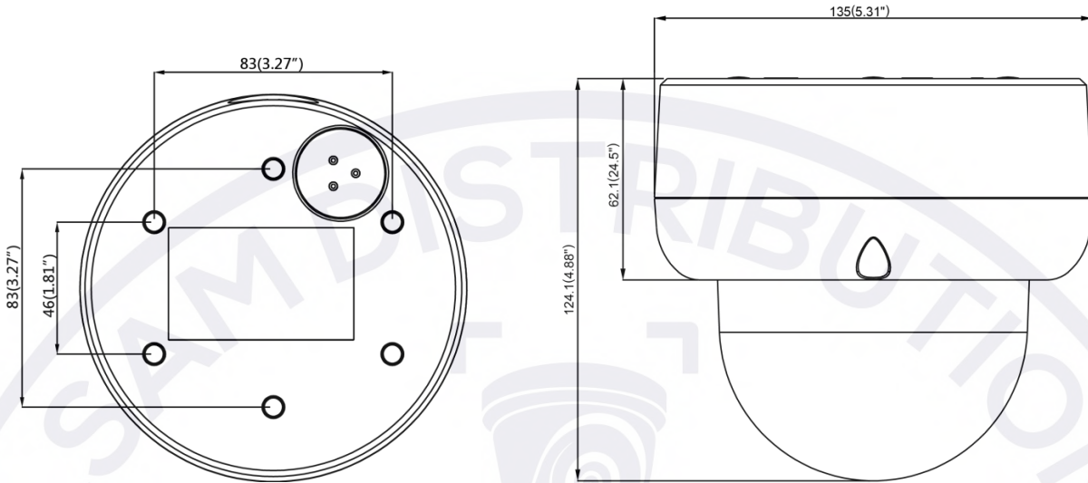
Figure 1 - 1: Physical Dimensions
