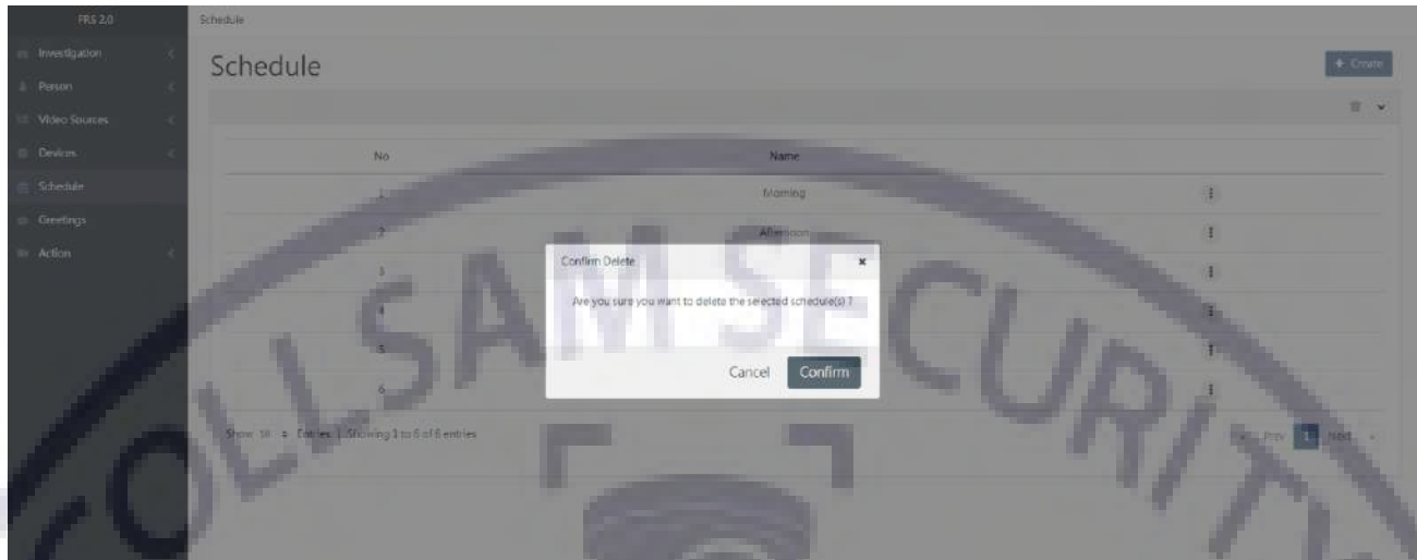
FIGURE 3.60 Delete Schedule
